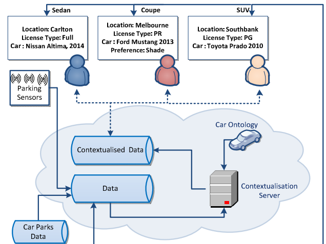
Fig. 2. Smart Parking
